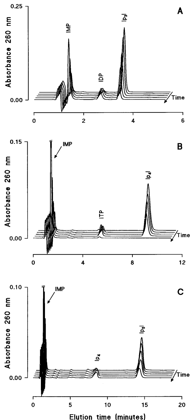
Fig. 2. Characterization of Ip X I through phosphodiesterase digestion. Putative Ip X I were incubated with phosphodiesterase from C. durissus , as described in Experimental Procedures. Aliquots taken at 0, 3, 6, 10, and 20 min were injected and analyzed by ion-pair chromatography to follow the Ip X I disappearance and the appearance of the corresponding degradation products. A, Characterization of Ip 3 I through digestion with phosphodiesterase. Putative Ip 3 I was treated as previously described. The consecutive chromatograms correspond to the HPLC profiles obtained at increasing digestion times. The disappearance of the Ip 3 I is concomitant with the appearance of peaks of their degradation products (IMP and IDP). B, Characterization of Ip 4 I through digestion with phosphodiesterase. Putative Ip 4 I was analyzed as described in A for Ip 3 I. The consecutive chromatograms show the formation of ITP and IMP from Ip 4 I through incubation at increasing times with phosphodiesterase. C, Characterization of Ip 5 I through digestion with phosphodiesterase. Putative Ip 5 I was treated in the manner described for Ip 3 I and Ip 4 I. Digestion of Ip 4 I peak with phosphodiesterase yields IMP and another metabolite with a retention time higher than that for ITP. This compound has been putatively identified as inosine-5'-tetrphosphate.
