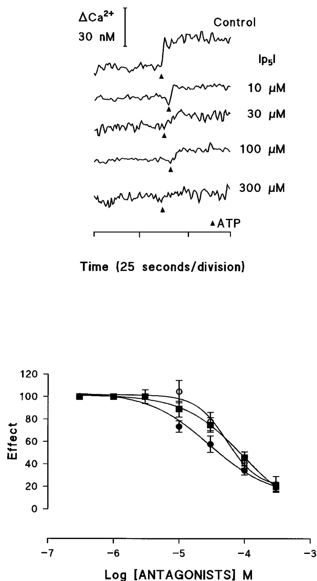
Fig. 6. Antagonistic effect of \text{Ip}_5\text{I} on the responses induced by ATP. A, Responses to ATP (100 \mu\text{M} ) in the presence of graded concentrations of \text{Ip}_5\text{I} . The antagonist was preincubated for 2 min before the application of the agonist, as described in Experimental Procedures. B, Inhibitory effect of \text{Ip}_n\text{Is} ( \blacksquare , \text{Ip}_3\text{I} ; \circ , \text{Ip}_4\text{I} ; \bullet , \text{Ip}_5\text{I} ) on the \text{Ca}^{2+} transients elicited by 100 \mu\text{M} ATP. Graded concentrations of the \text{Ip}_n\text{Is} were added to obtain the corresponding responses, which were attenuated in the presence of higher doses of the antagonists. Ordinates, \text{Ca}^{2+} transients as a percentage of the control value for 100 \mu\text{M} ATP in the absence of any substance. Values are mean \pm standard error from four experiments performed in duplicate.
