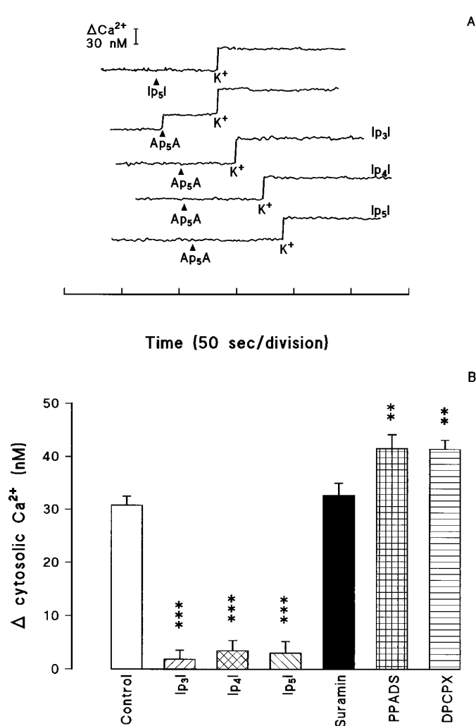
Fig. 3. Antagonistic effect of \text{Ip}_n\text{Is} and purinergic antagonists on \text{P}_4 purinoceptors present in rat brain synaptic terminals. A, Effects of \text{Ip}_3\text{I} , \text{Ip}_4\text{I} , and \text{Ip}_5\text{I} on calcium entry into rat brain synaptosomes evoked by 100\ \mu\text{M} \text{Ap}_5\text{A} . Effects of \text{Ip}_5\text{I} and \text{Ap}_5\text{A} on \text{Ca}^{2+} responses induced through the dinucleotide receptor (top two traces). The effect of \text{Ap}_5\text{A} was blocked by the three \text{Ip}_n\text{Is} applied at a final concentration of 100\ \mu\text{M} (bottom three traces). B, Comparative behavior of \text{Ip}_n\text{Is} and purinergic antagonists. All compounds were assayed at a final concentration of 100\ \mu\text{M} , except DPCPX, which was applied at a concentration of 250\ \text{nM} , modifying the \text{Ap}_5\text{A} response in a different way. All experiments represent the mean \pm standard error of four different experiments performed in duplicate. **, p < 0.01 versus control; ***, p < 0.001 versus control.
