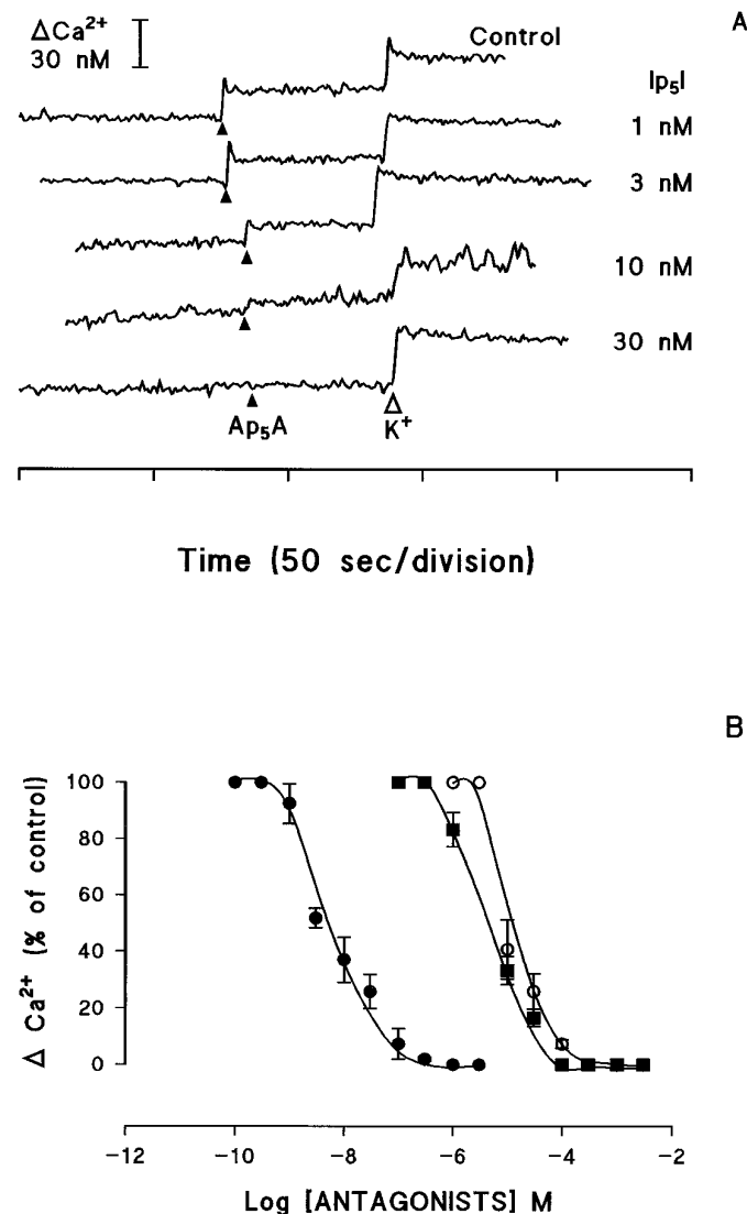
Fig. 4. Effects of \text{Ip}_n\text{Is} on the responses elicited by 100\ \mu\text{M} \text{Ap}_5\text{A} . A, Increasing doses of \text{Ip}_5\text{I} produced a gradual blocking of the responses elicited by \text{Ap}_5\text{A} . A 30\ \text{mM} \text{K}^+ pulse is given at the end of each record as a control of the synaptosomal functional response. B, Effect of (■) \text{Ip}_3\text{I} , (○) \text{Ip}_4\text{I} , and (●) \text{Ip}_5\text{I} on the \text{Ca}^{2+} transients elicited by 100\ \mu\text{M} \text{Ap}_5\text{A} . Graded concentrations of the \text{Ip}_n\text{I} were added to obtain the corresponding responses. Ordinates, \text{Ca}^{2+} transients as a percentage of the control value for 100\ \mu\text{M} \text{Ap}_5\text{A} in the absence of any substance. Values are mean \pm standard error from four experiments performed in duplicate.
